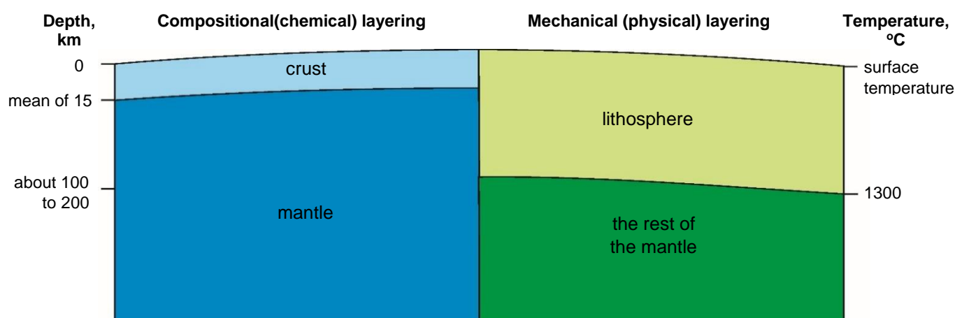
Figure 4.12. The outer part of the Earth
