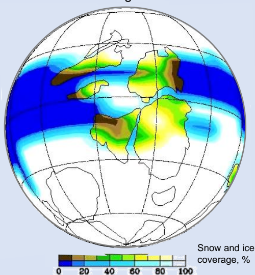
Computer simulation of ice coverage during Snowball Earth
