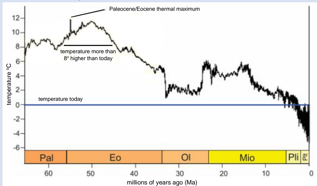
Temperature of Earth (°C) compared with today's temperature, over the past 65 Ma
