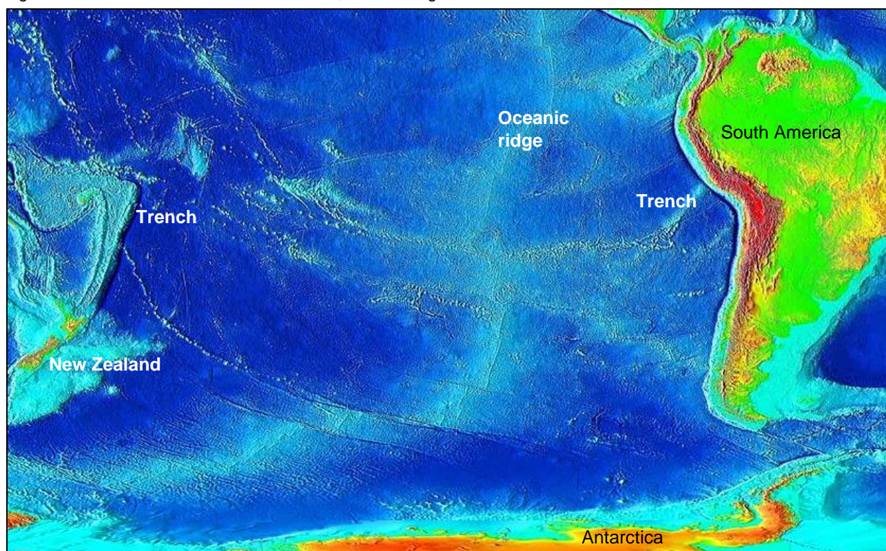
Figure 4.13. The southern Pacific Ocean floor; oceanic ridge near the centre and trenches to East and West
