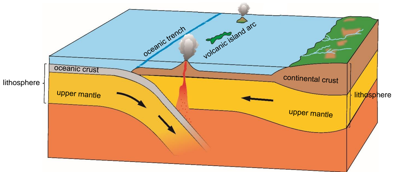
Figure 4.24. Subduction at a collision of two oceanic plates
