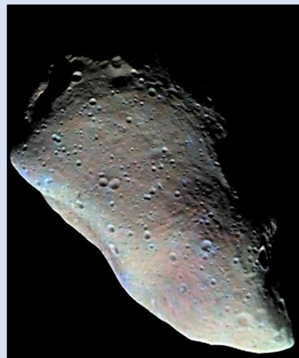
Asteroid Gaspra photographed from the Galileo spacecraft
