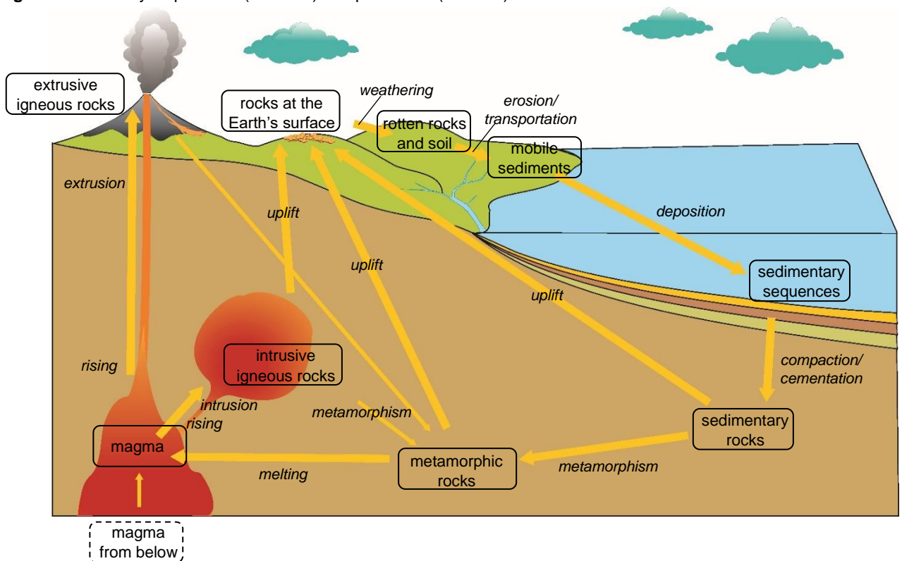
Figure 1.7. Rock cycle products (in boxes) and processes ( in italics ).
