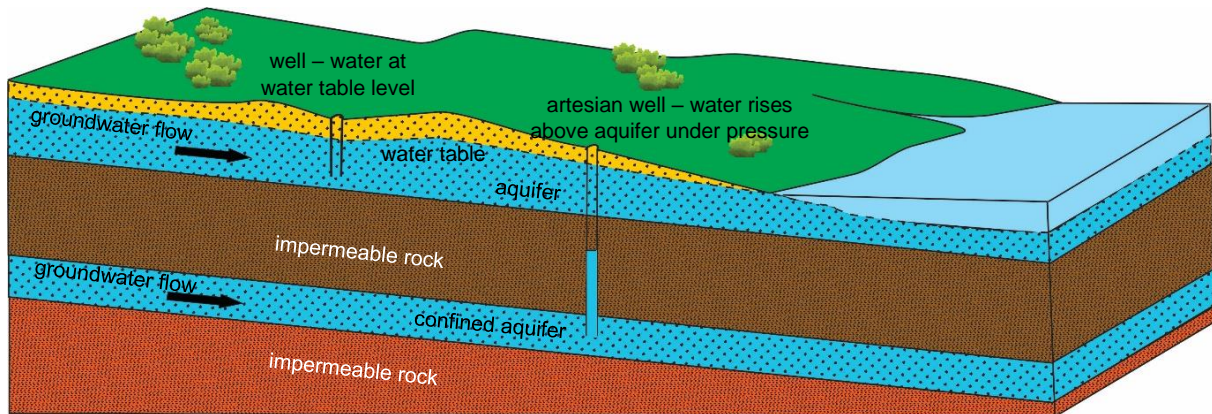
Figure 4.36. Aquifers
