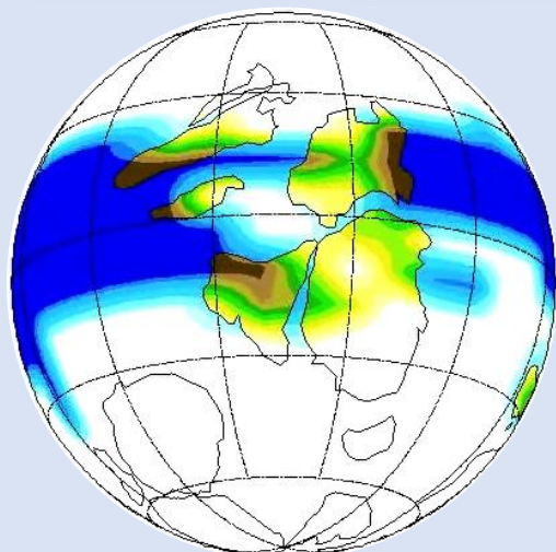
Computer simulation of ice coverage during Snowball Earth
