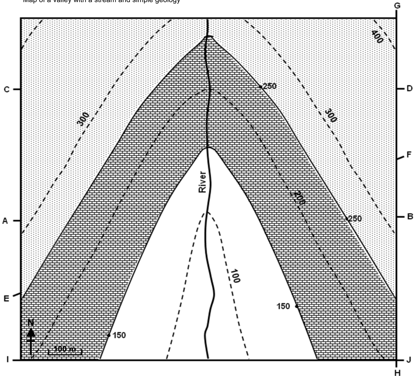
Map of a valley with a stream and simple geology
