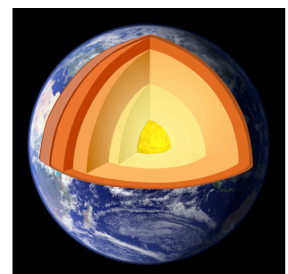
The Earth's core - shown in yellow.
